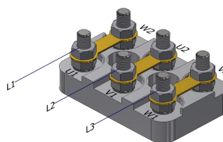
Three - phase connection Triangle connection
